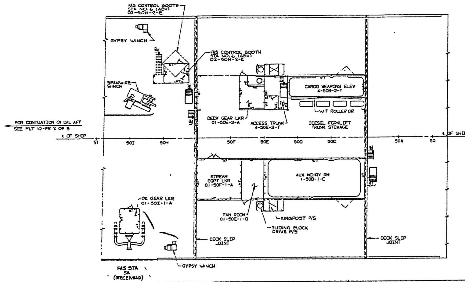
01 LEVEL MIDBODY NAVSEA 801-5183615 PLATE NO. 10-FR 3 OF 3
