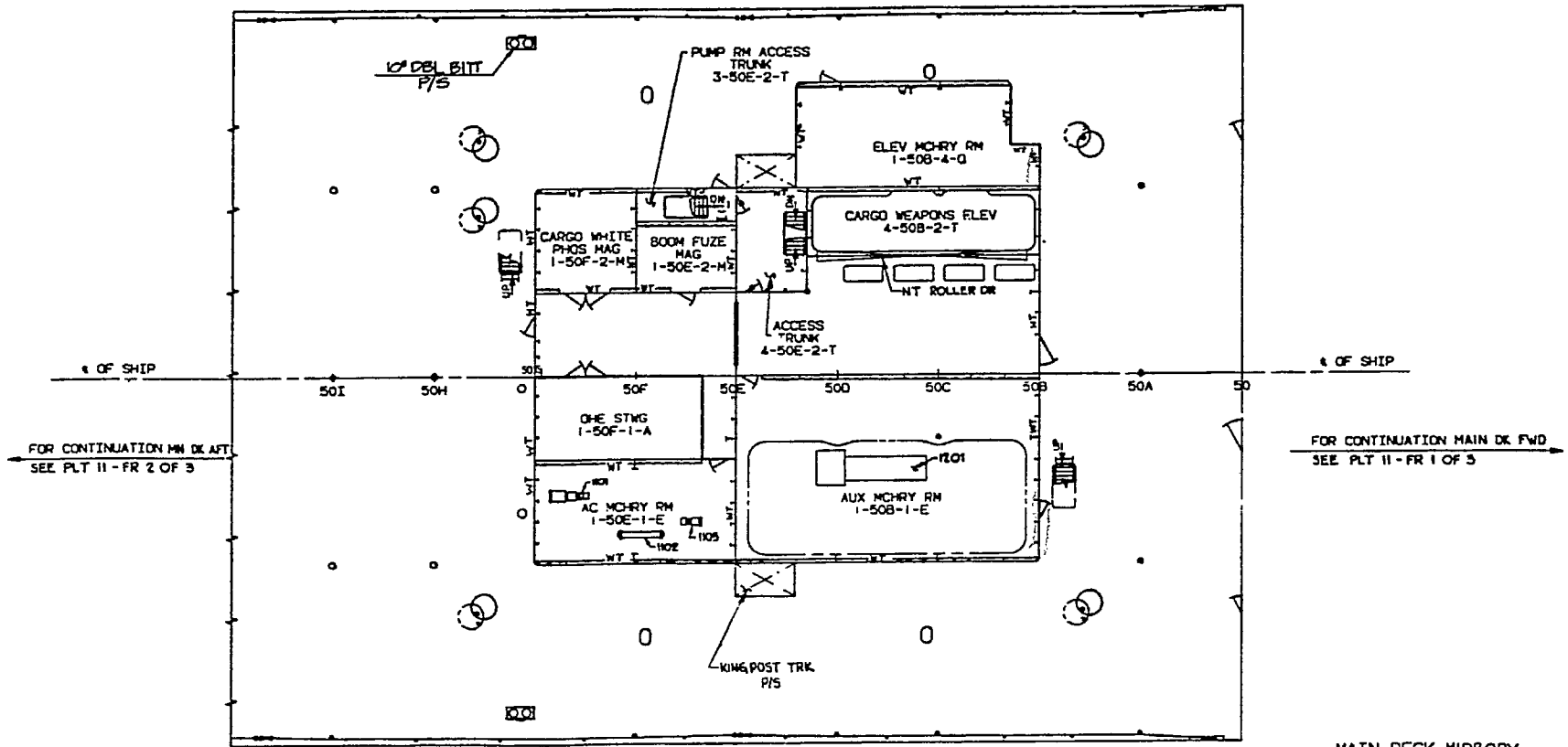
MAIN DECK MIDBODY NAVSEA 801-5183615 PLATE NO. 11 FR 3 OF 3
