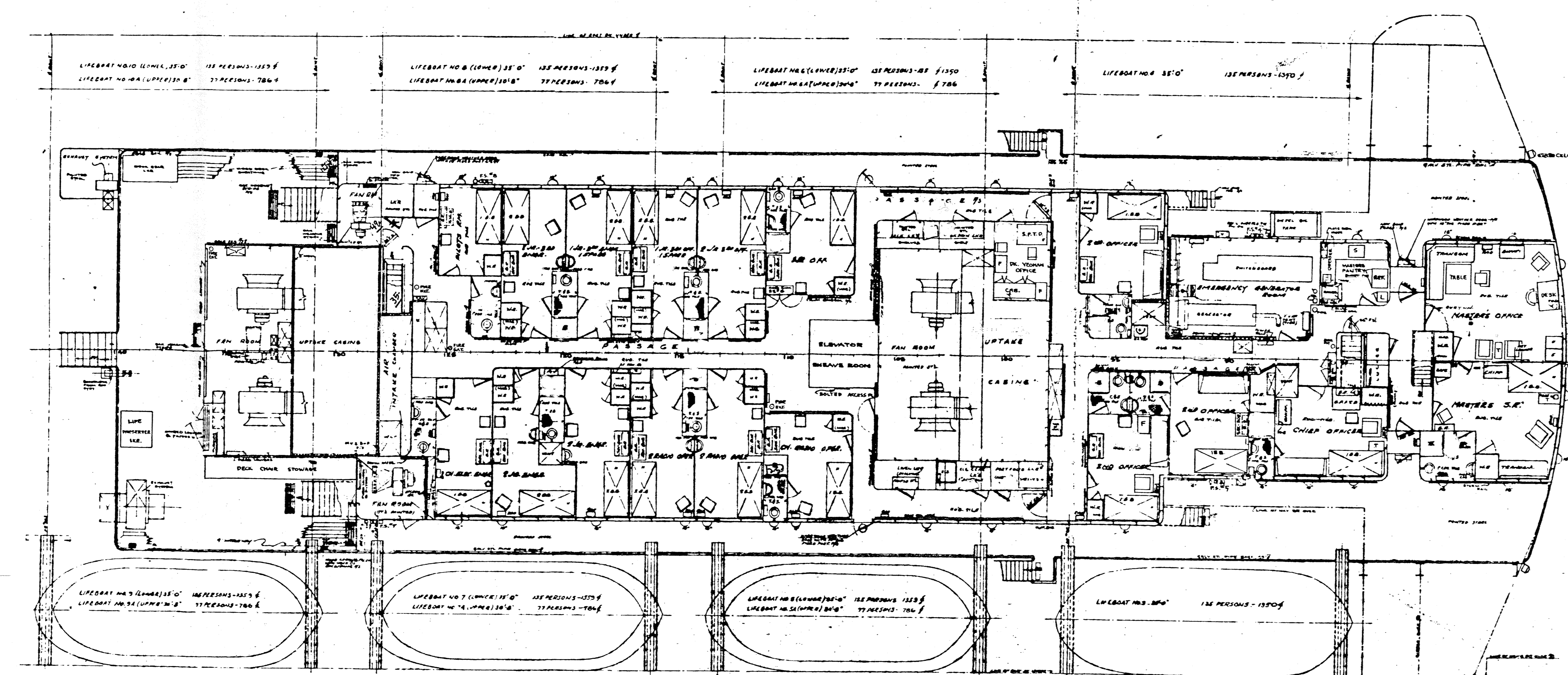
BRIDGE DECK 56 ISL Level # 2 Vessel Level 02
