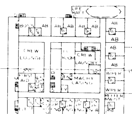
BOAT DECK 81' 6" ABV BL
