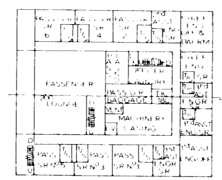
CABIN DECK 90' 6" ABV BL
