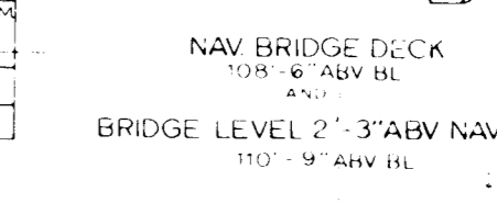
BRIDGE LEVEL 2'-3" ABV NAV BR DK 110'-9" ABV BL
