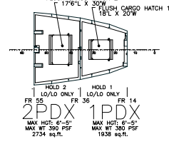
PLATFORM DECK (PDX) TOTAL LO/LO AREA = 4,672 SQ FT
