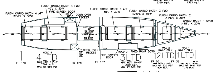
FIRST PLATFORM (LTD) TOTAL LO/LO AREA = 2,361 SQ FT TOTAL RO/RO AREA = 14,969 SQ FT
