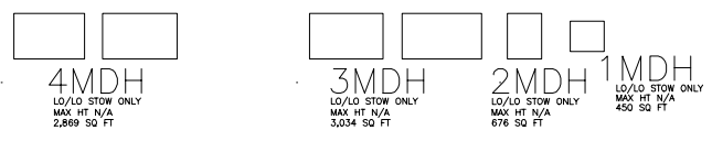
MAIN DECK HATCHES (MDH)
