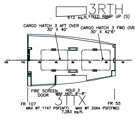
TANK TOP (TTX) TOTAL RO/RO AREA = 7,895 SQ FT RAMP SQ FT INCLUDED IN RO/RO AREA
