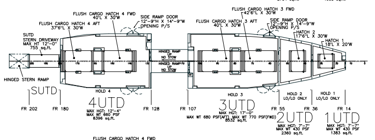
SECOND DECK (UTD) TOTAL LO/LO AREA = 3,743 SQ FT TOTAL RO/RO AREA = 17,683 SQ FT
