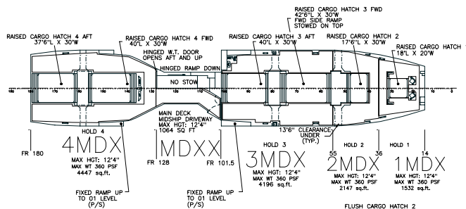
MAIN DECK (MDX) TOTAL LO/LO AREA = 7,029 SQ FT TOTAL RO/RO AREA = 13,386 SQ FT
